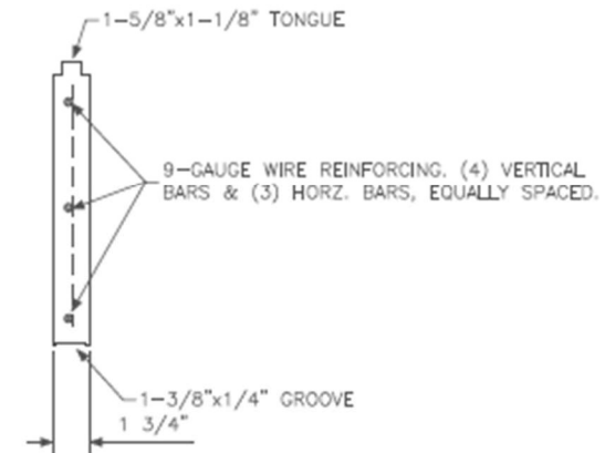
WALL PANEL - SECTION
