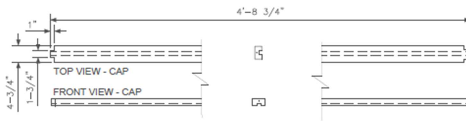
WALL PANEL CAP - PLAN VIEW & ELEVATION
