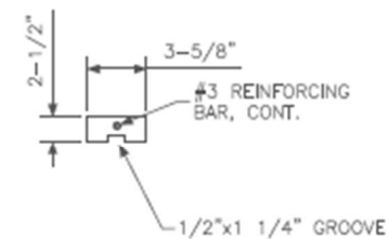
WALL PANEL CAP - SECTION
