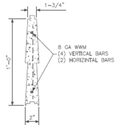
WOODCRETE® PANEL - SECTION
