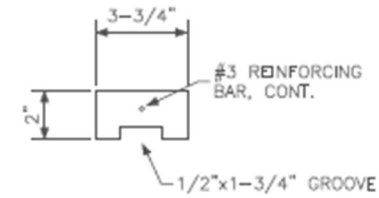
WOODCRETE® CAP - SECTION
