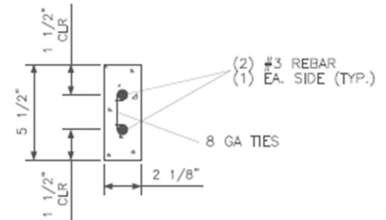
RAIL SECTION
