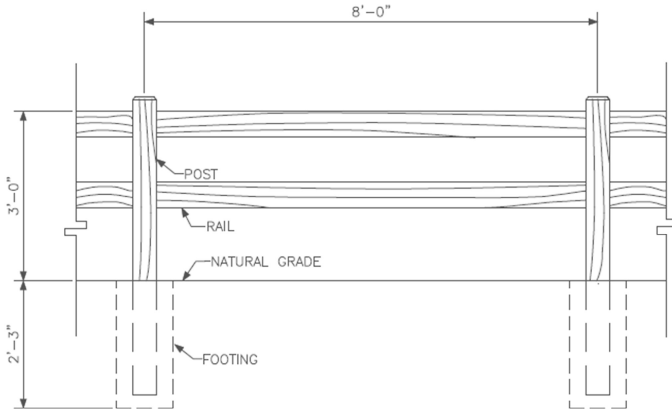
ELEVATION - 2 RAIL FENCE
