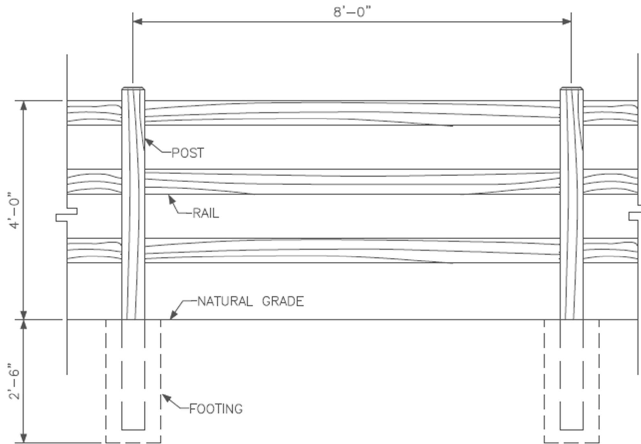
ELEVATION - 3 RAIL FENCE
